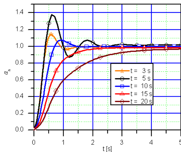
Figure 5 – Responses of a conventional autopilot designed for t=10 s
