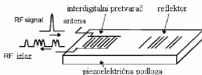
Slika 3 – Šematski prikaz refleksionog PAT filtra Figure 3 – Schematic presentation of the reflection SAW filter
