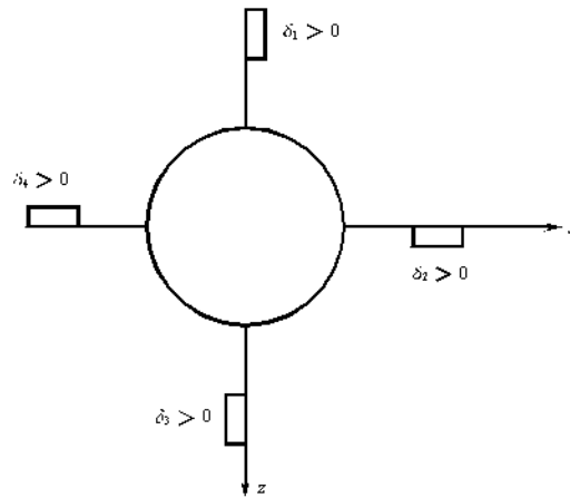
Figure 5 – Positive deflections of the fins (rear view).
