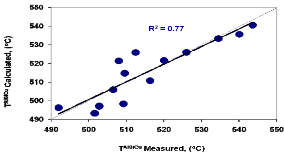
Figure 6 - Calculated versus measured Al-Si-Cu eutectic nucleation temperature using equation (8)
