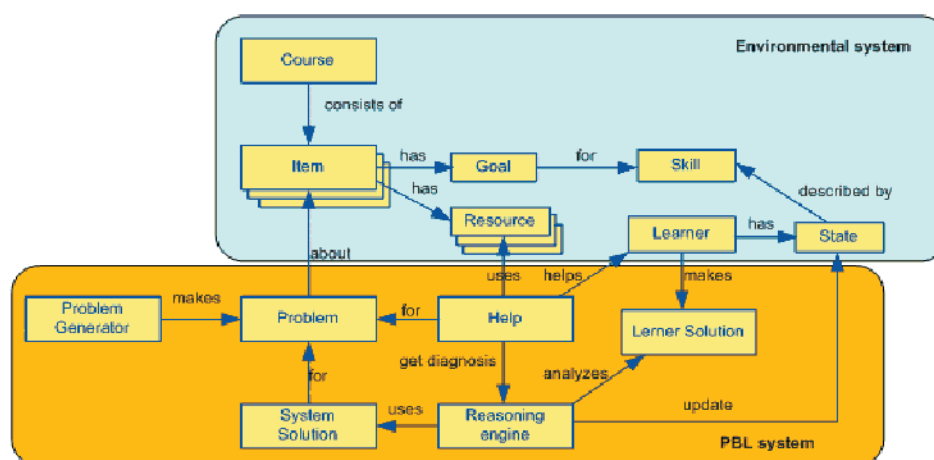
Figure 1 – The additional concepts which improve contextual help
