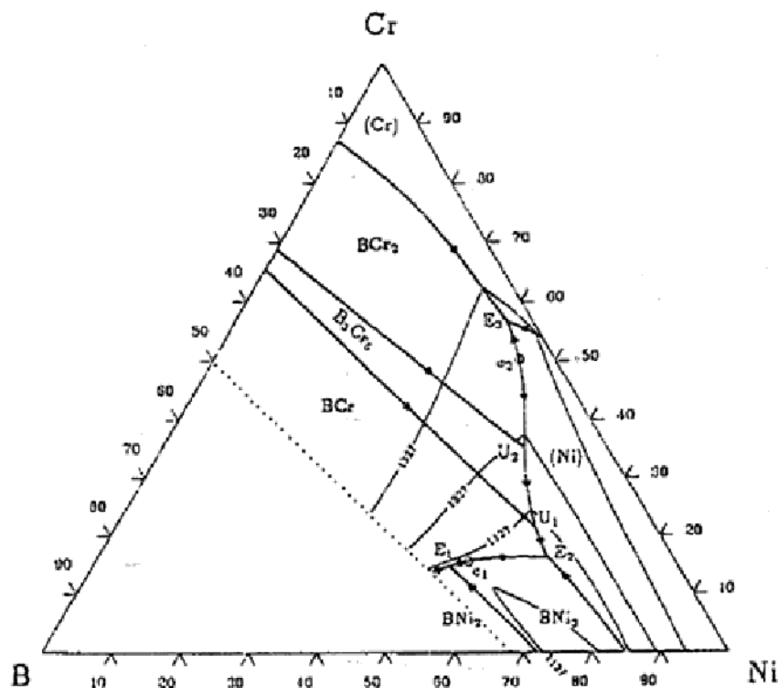
Figure 1 - Ternary phase diagram of Ni-Cr-B alloy [8] Slika 1 - Ternarni sistem Ni-Cr-B [8]
