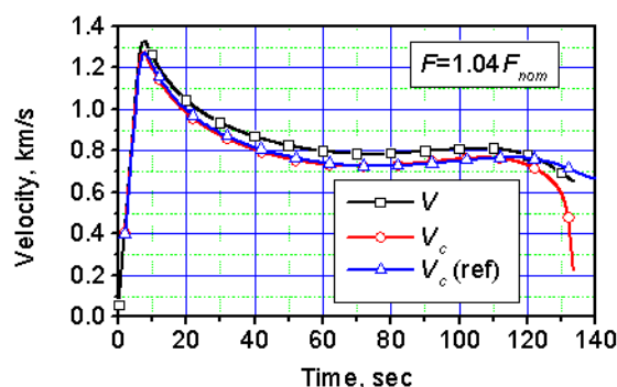
Figure 11 – Missile velocity and correlated velocity vs time.
