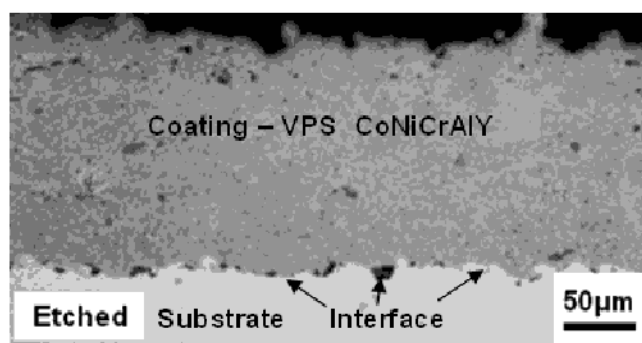
Figure 8 – Etched microstructure of the \text{Co}_{32}\text{Ni}_{21}\text{Cr}_8\text{Al}_{10.5}\text{Y} coating deposited on the sample with a substrate distance of 270 mm
