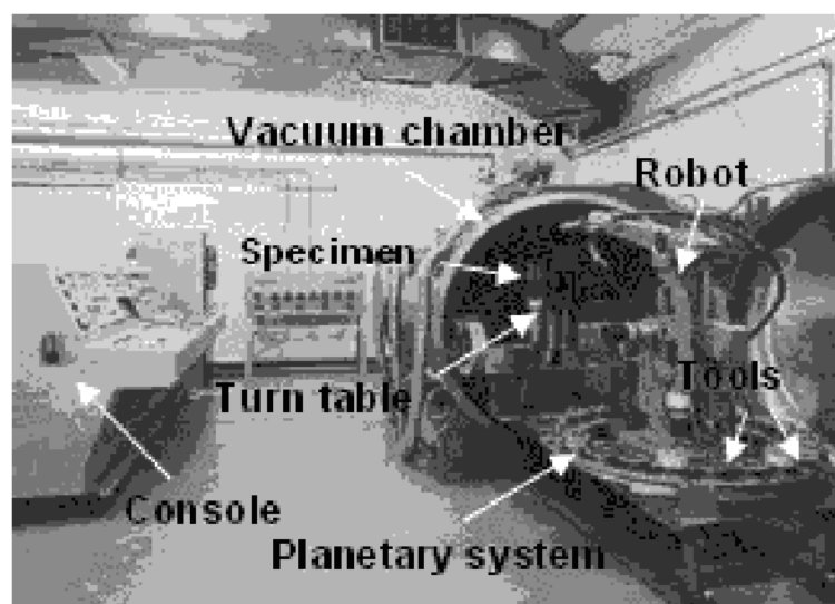
Figure 2 – Vacuum plasma spray system Slika 2 – Vakuim plazma sprej sistem
